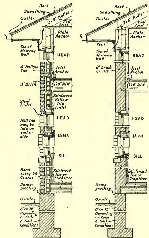
Wall Sections
